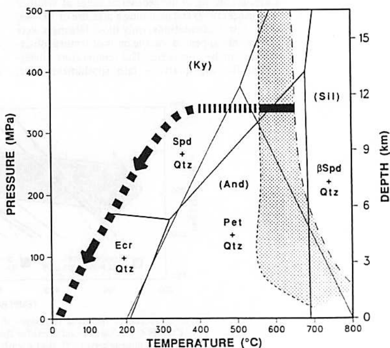
FIG. 6. Pressure - temperature path (bold curve) for the magmatic crystallization (solid line), hydrothermal stage (short-dashed line) and uplift (long-dashed curve) of the Harding pegmatite. Selected equilibria from Figures 1 and 2 also are shown and include the aluminosilicate phase diagram (solid lines), the Li-Al-silicate phase diagram (bold solid lines), and the liquidus (short-dashed line) and solidus (long-dashed line) of the water-saturated Harding pegmatite magma. The region of magmatic crystallization is shaded. See Figures 1 and 2 for references.
